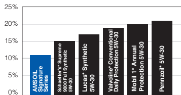
VISCOSITY BREAKDOWN Represented By % Viscosity Lost In The Kurt Orbanh Test
